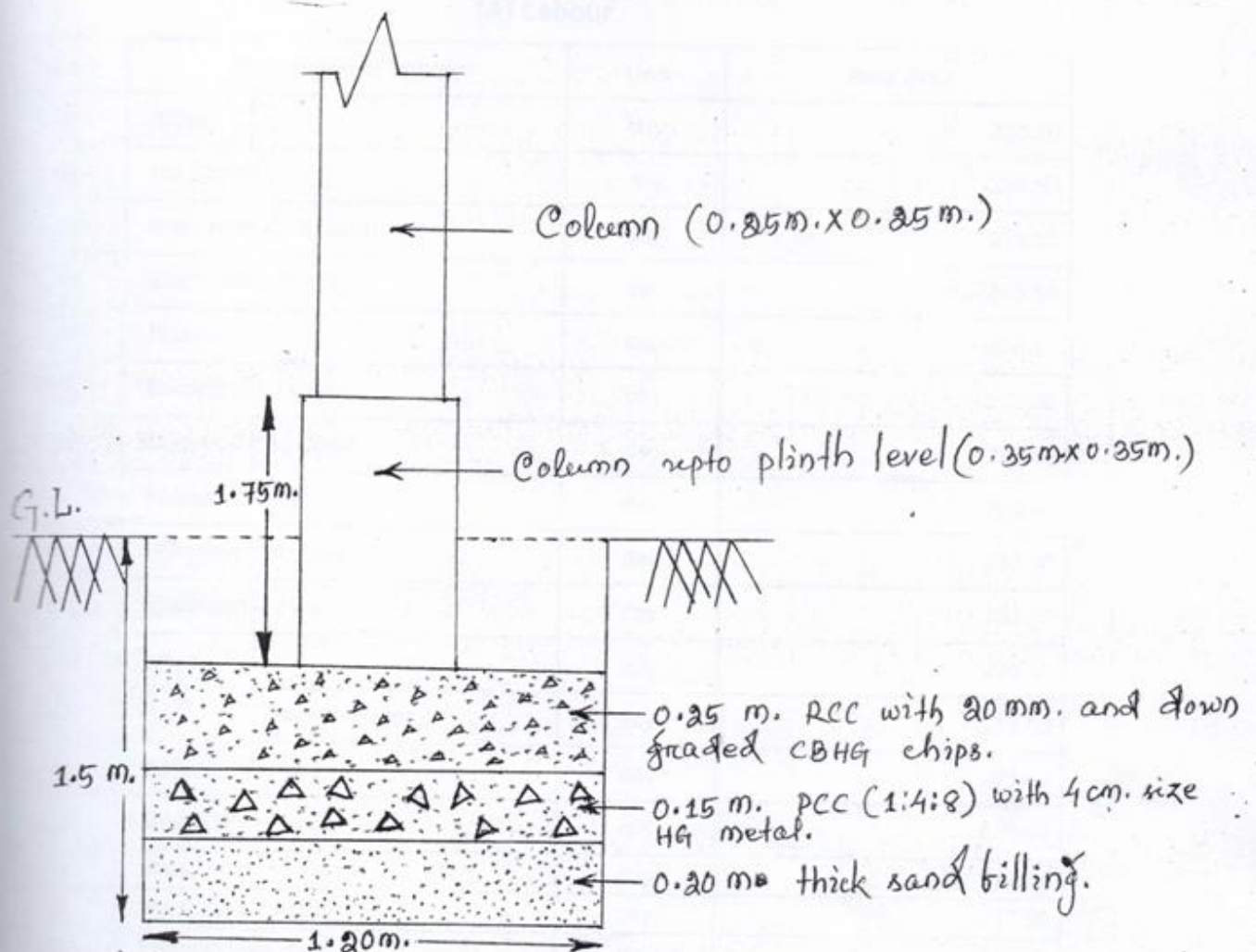
CROSS-SECTION OF COLUMN
