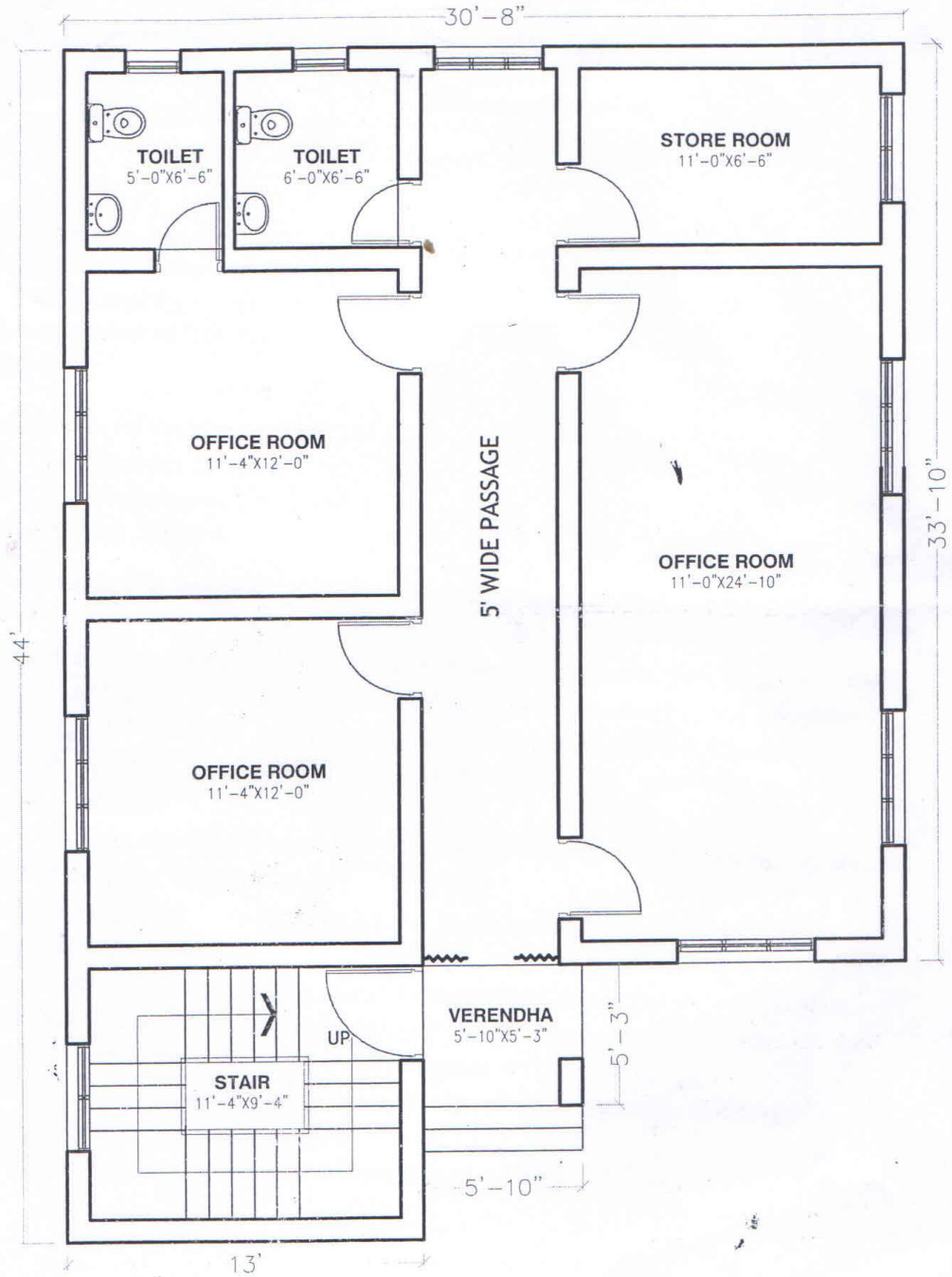
GROUND FLOOR PLAN PLINTH AREA-1200 SFT
