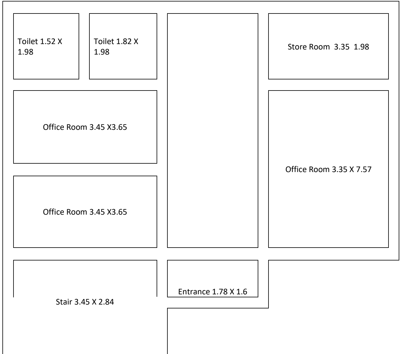
PLAN GROUND FLOOR
