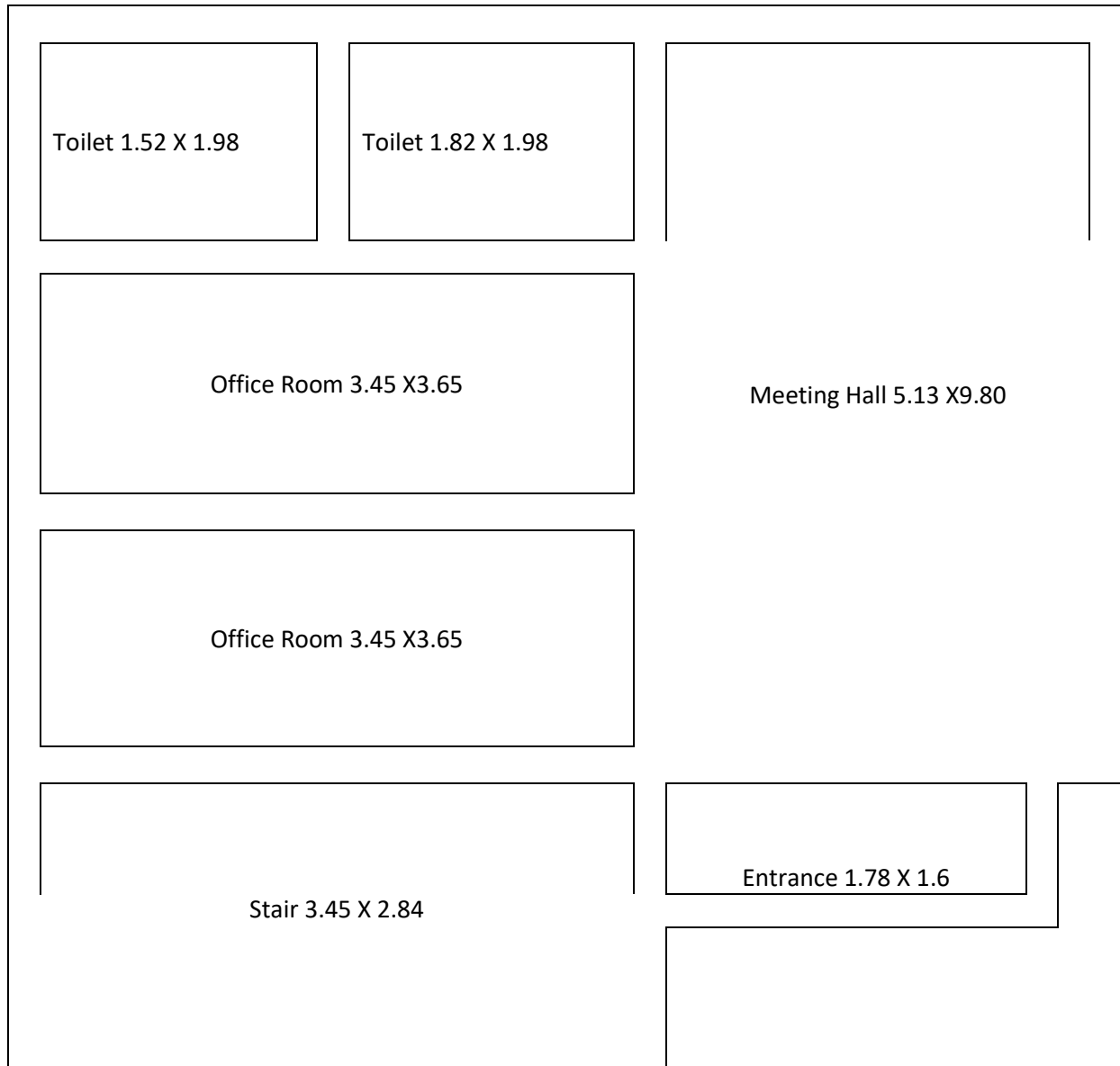
PLAN FIRST FLOOR
